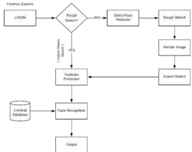
Fig. 7. Flow Chart for Creating a sketch in the application
