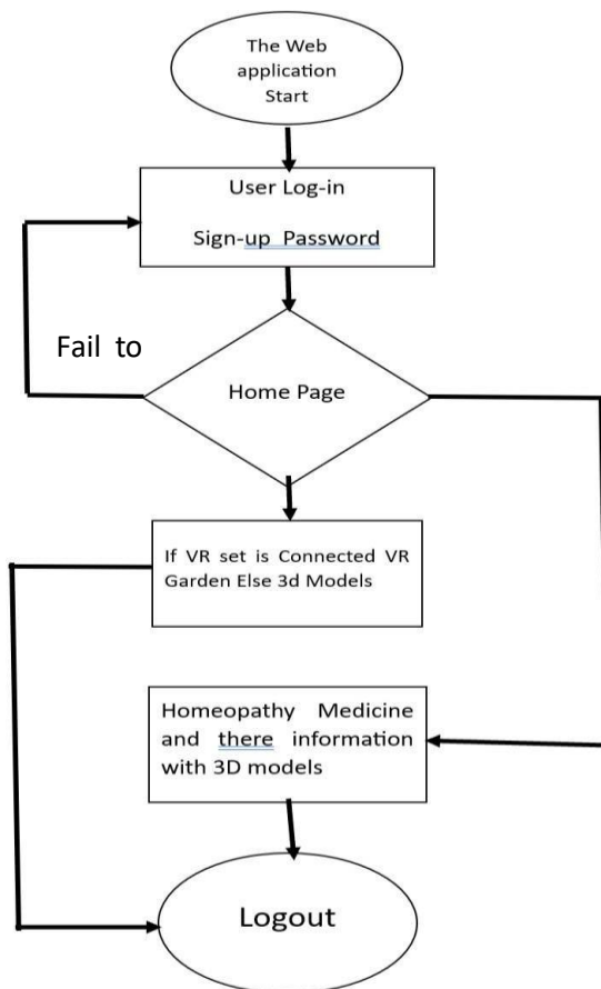
Figure 5.1: Flow Diagram
