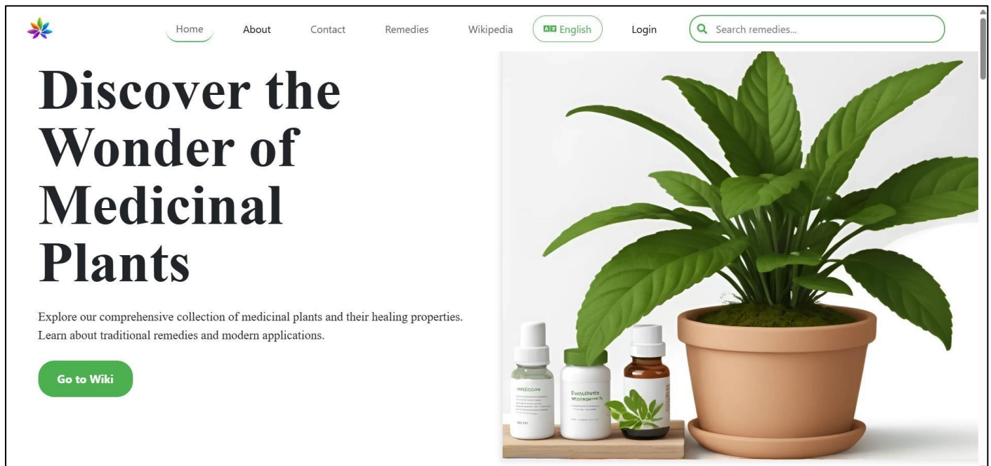
Figure1: Home Page
