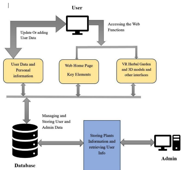
Figure 5.2: System Architecture
