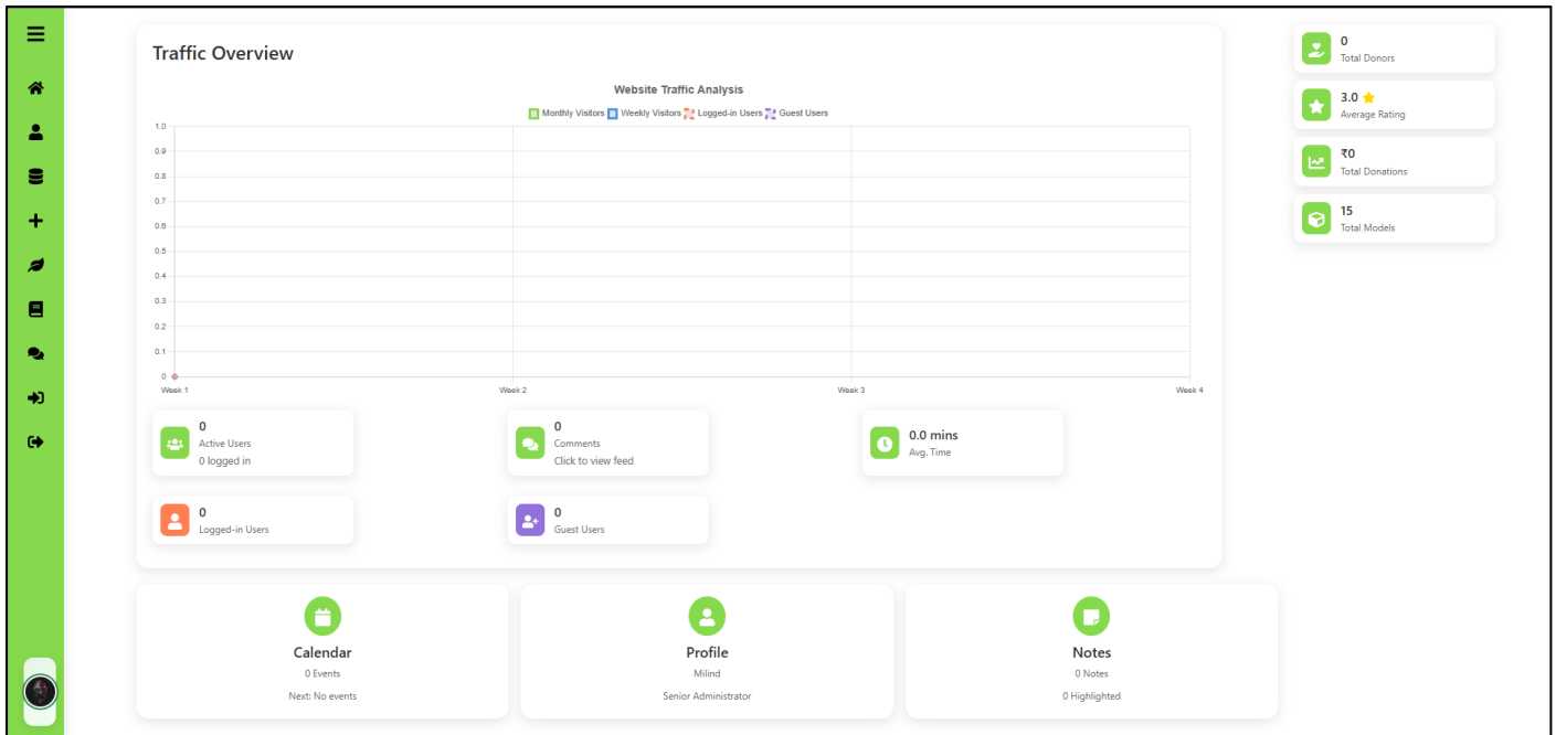
Figure5: Admin
