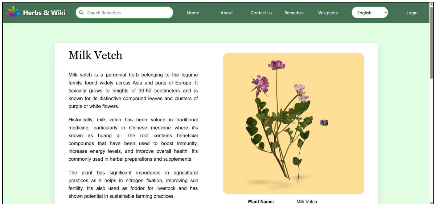
Figure3: Herbs Page
