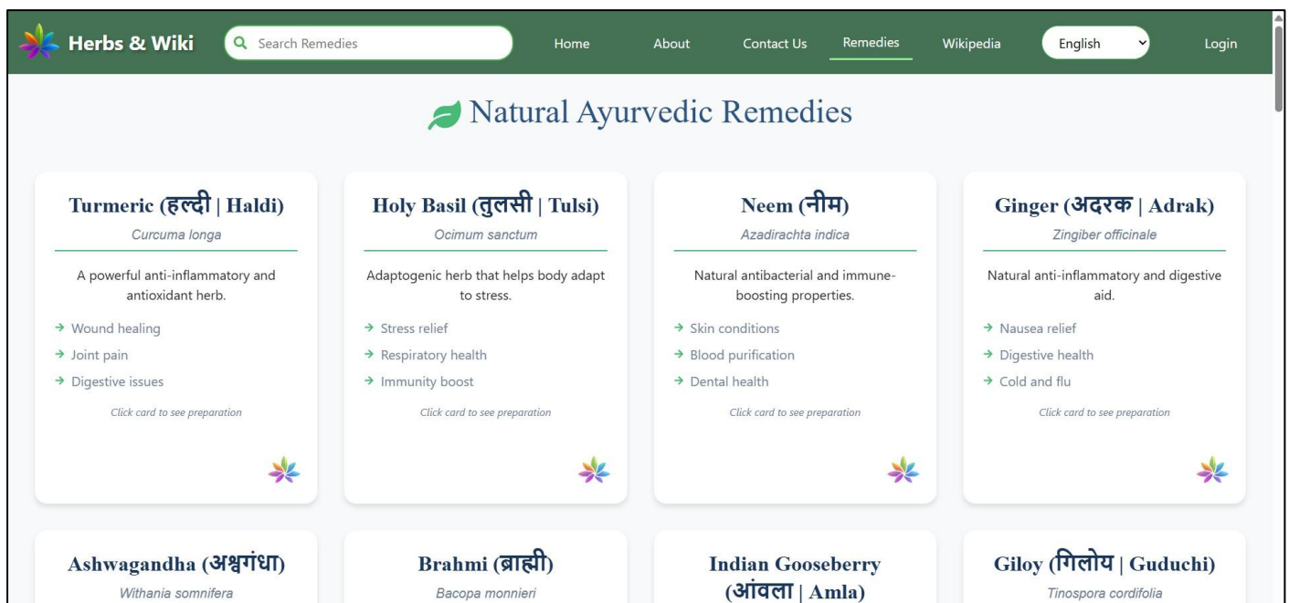
Figure2: Remedies
