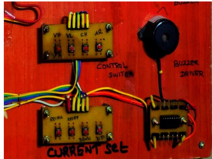
Fig 8.3 Hardware module for Control Unit and Alarm Unit
