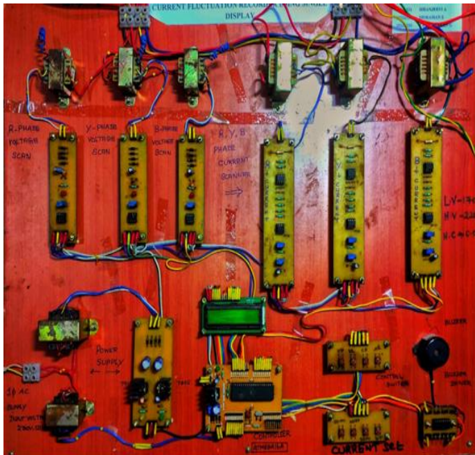
Fig 8.1 Hardware module for R, Y, B 3Phase Scanner
