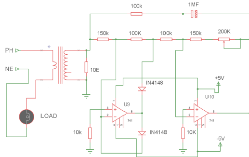
Fig 6.1 Current Measurement
