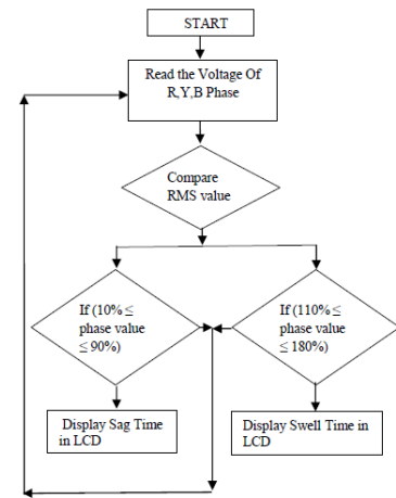
Fig 6.3 Flow Chart for R,Y, B PHASE Scanner
