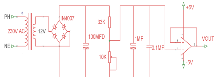
Fig 6.2 Voltage Measurements
