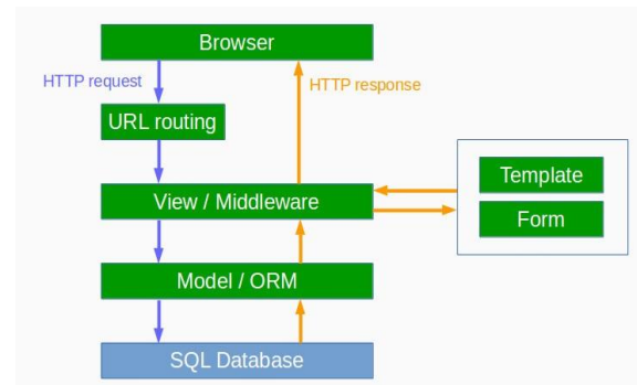
Figure 2.3.7: Architectural view of Django
