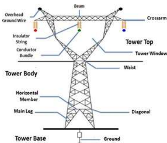
Fig.2: Transmission line tower
