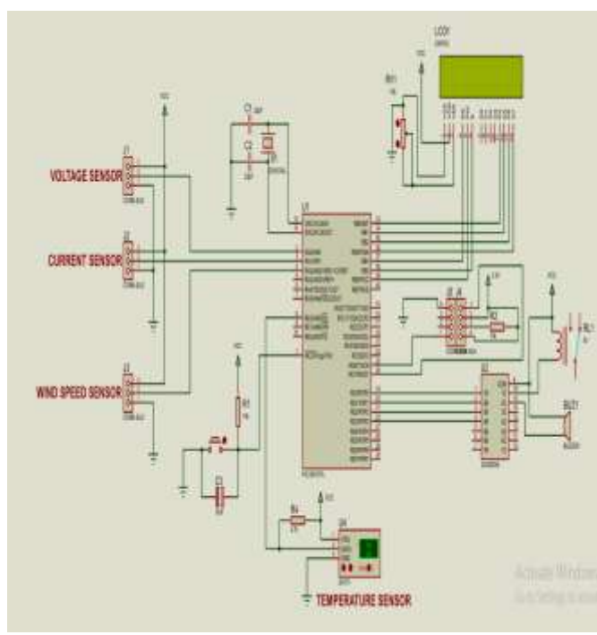
Circuit diagram of Simulation in Proteus
