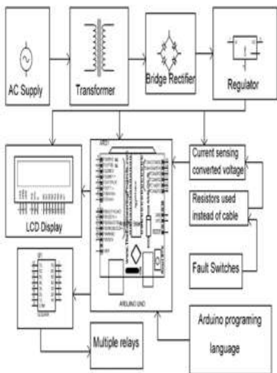
Fig.3: Circuit Diagram
