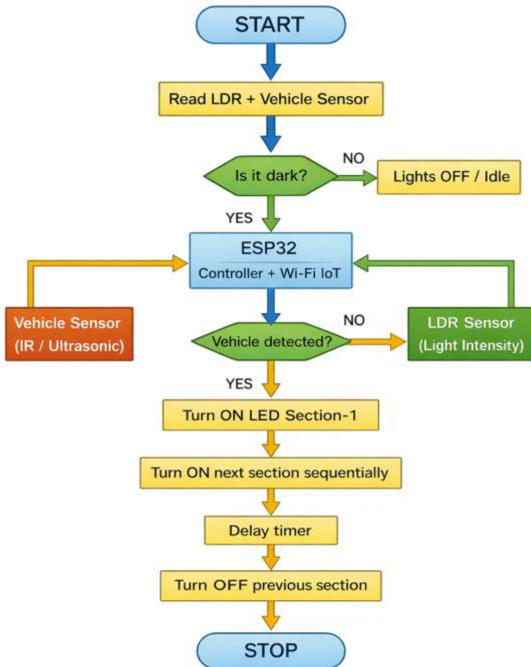
Fig. 2: Flowchart of System Working
