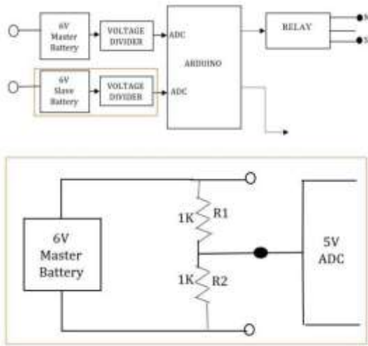
Fig 3.3 BMS of Master and Slave Battery
