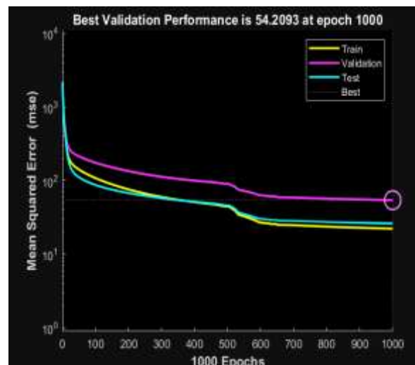
Fig.4 Training Convergence
