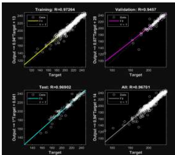
Fig.6 Regression Analysis
