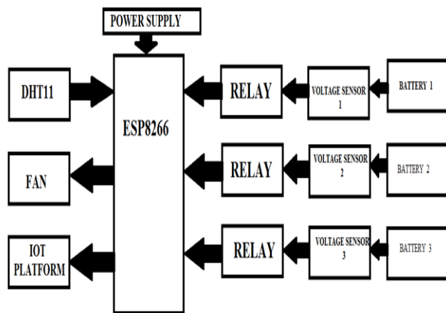
Fig 2: Block Diagram of IoT based BMS.
