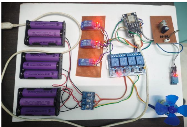
Fig 3: Hardware of IOT Based BMS
