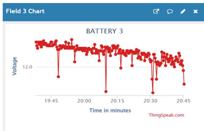
Fig :6 Photocopy of voltage graph of battery 3 with load (fan) using IOT
