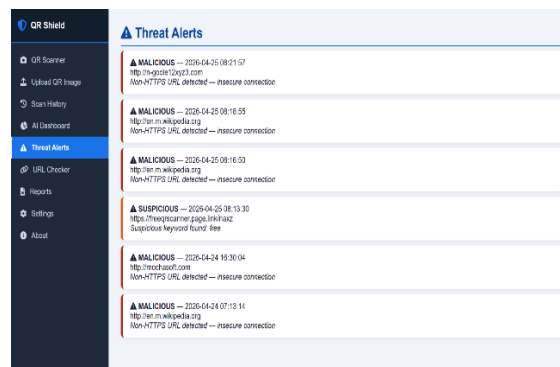
Fig-5: Real-time threat alert validation interface isolating unencrypted malicious payloads and insecure network connections
