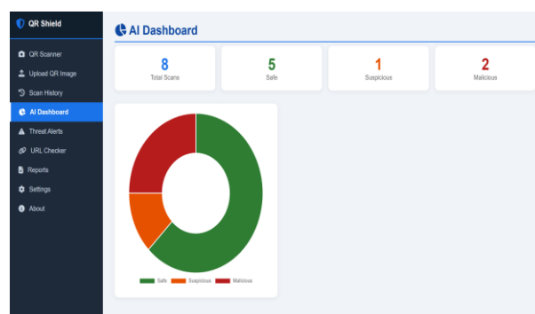
Fig-3: Visual Dashboard Interface for monitoring and threat category tracking
