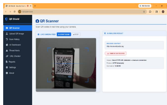
Fig-4: Secure Result Presentation Interface for displaying defensive workflow and visual hazard notifications.
