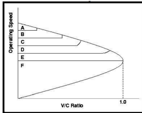
Figure 12 Level of Service
