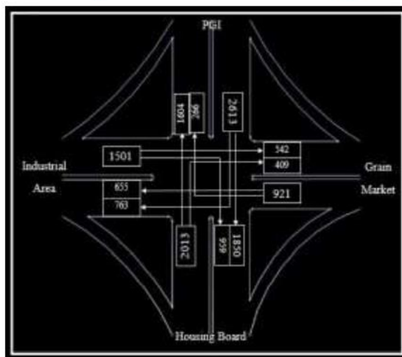
Figure 9 Traffic Flow Diagram for the Peak Hour Flow
